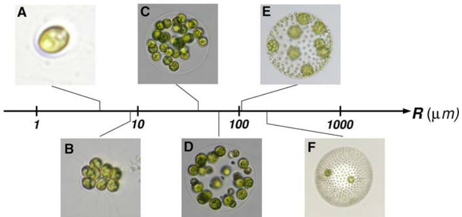
Fig. 1 Volvoclean green algae arranged according to typical colony radius R . The lineage ranges from the single-cell Chlamydomonas reinhardtii (A), to undifferentiated Gonium pectorale (B), Eudorina elegans (C), to the soma-differentiated Pleodorina californica (D), to the germ-soma differentiated Volvox carteri (E), V. aureus (F), and even larger (e.g., V. gigas with a radius of 1 mm). In species in which two cell types can be identified, the smaller are somatic cells and the larger are reproductive cells. Note that the number of cells in Volvox species ranges from 1,000 (e.g., V. carteri ) to 50,000 (e.g., V. barberi )
