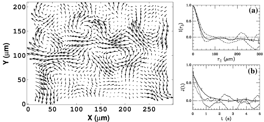
Fig. 5 Results from PIV studies of collective behavior in bacterial suspensions [22]. Left: vector field of swimming patterns, and correlation functions in space (a) and time (b)
