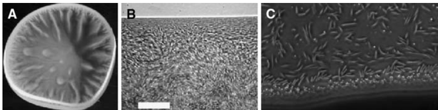
Fig. 4 Three scales of organization in suspensions of B. subtilis . (A) bioconvection in a sessile drop of diameter 1 cm [22]. (B) close-up of collective swimming in the ZBN near the contact line. Blurring arises from very fast swimming speed. Scale bar is 35 \mu\text{m} . (C) even closer view at lower concentration and in a shallow layer, showing accumulation at the contact line and 0.5 \mu\text{m} fluorescent microspheres used for flow tracers
