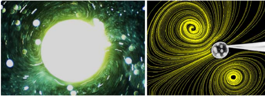
Fig. 3 Flow fields around Volvox carteri colonies approximately 300 microns in diameter. Left panel is a time exposure of several seconds which reveals the complex flows of tracers near the colony surface. Right panel shows streamlines obtained from a time series of many tens of seconds around a colony held fixed with a glass micropipette
