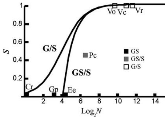
Fig. 2 Results of the hydrodynamic model: Proportion s of somatic cells needed by colonies of C. reinhardtii -type cells to avoid sinking. Model results for colonies with unspecialized reproductive cells (GS) and soma (S; GS/S colonies) and for colonies with specialized germ (G) and soma (G/S colonies) are plotted as a function of number of cell divisions ( \text{Log}_2N ). When s = 0 , colonies only have undifferentiated GS cells. For colonies to avoid sinking as they increase in size, they must invest in a higher proportion s of somatic cells. Note that for smaller colonies, GS/S colonies need a smaller proportion of somatic cells than G/S colonies to stay afloat since GS cells are flagellated. As size increases, the difference between the two colony types becomes negligible because the proportion (1-s) of reproductive cells becomes very small. Some of the extant species data is plotted to show how it fits with the model. Cr: C. reinhardtii ; Gp: G. pectorale ; Ee: E. elegans ; Pc: P. californica ; Vo: V. obversus ; Vc: V. carteri ; Vr: V. rousseletii . GS: undifferentiated colonies; GS/S: soma differentiated colonies; G/S: germ-soma differentiated colonies. Although V. rousseletii colonies reproductive cells start as flagellated cells, their flagella have essentially no motility function since they are reabsorbed before the first cell division. Thus, we consider V. rousseletii reproductive cells non-flagellated (G) and V. rousseletii G/S colonies. Figure adapted from Solari et al. [28]
